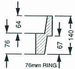
LIFTER RINGS DETAILS
